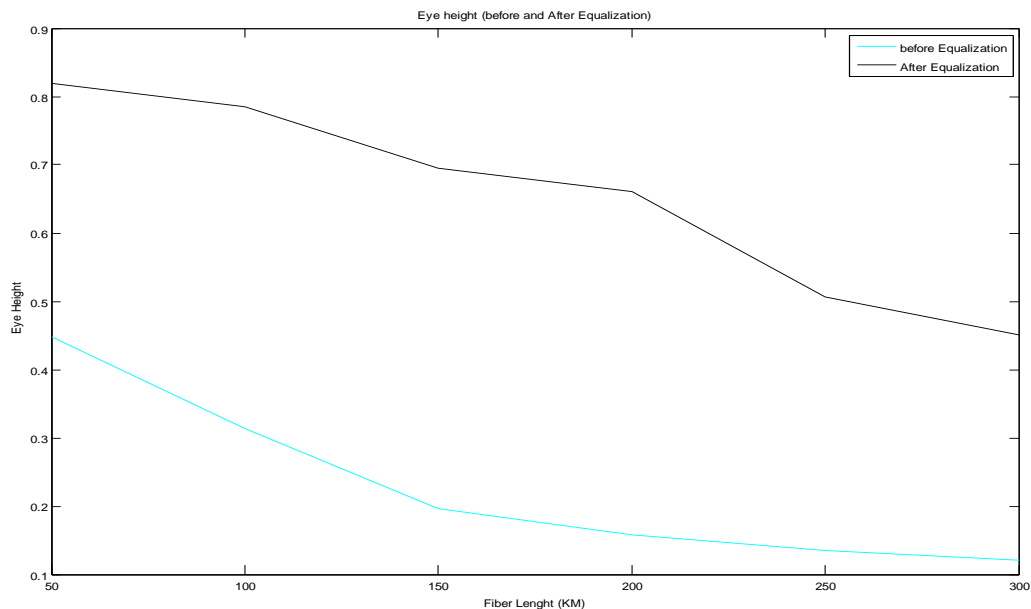
Fig. 13: Comparison Graph of Eye Height Vs Length of Fiber before and after equalization
